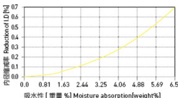
Graph HPP28-9: Effect of moisture absorption on HPP28 bearings
