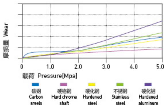
图表 HPP28-8: 旋转磨损随轴材料与压力变化关系 v=0.2\text{m/s} Graph HPP28-8: The bearing wear & pressure under rotating with different shaft materials, v=0.2\text{m/s}
