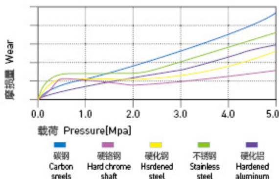
图表 HPP25-8: 旋转磨损随轴材料与压力变化关系 v=0.2\text{m/s} Graph HPP25-8: The bearing wear & pressure under rotating with different shaft materials, v=0.2\text{m/s}
